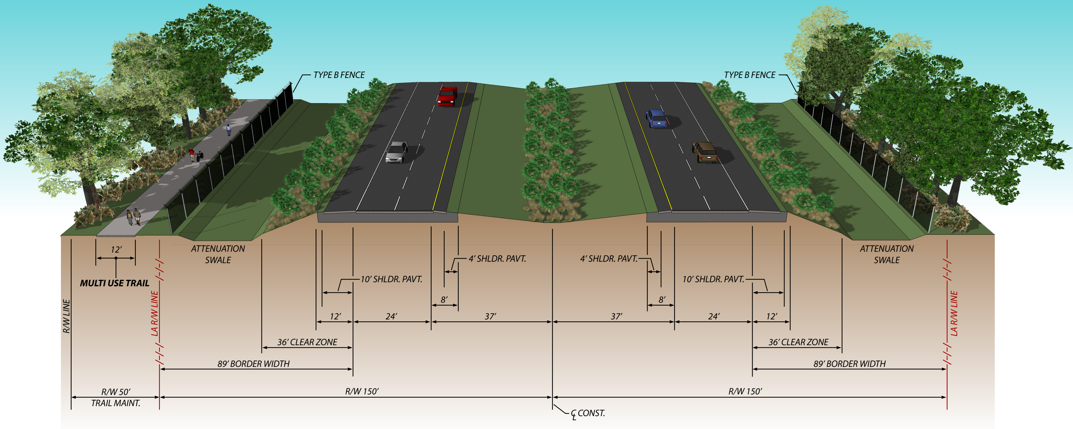
TYPICAL SECTION SUNCOAST PARKWAY SR 589
