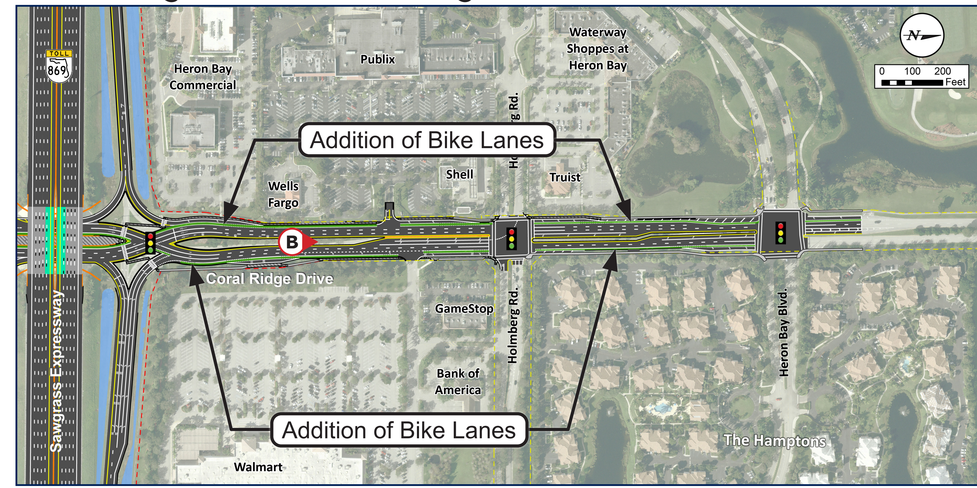
Coral Ridge Drive Interchange – North Section
