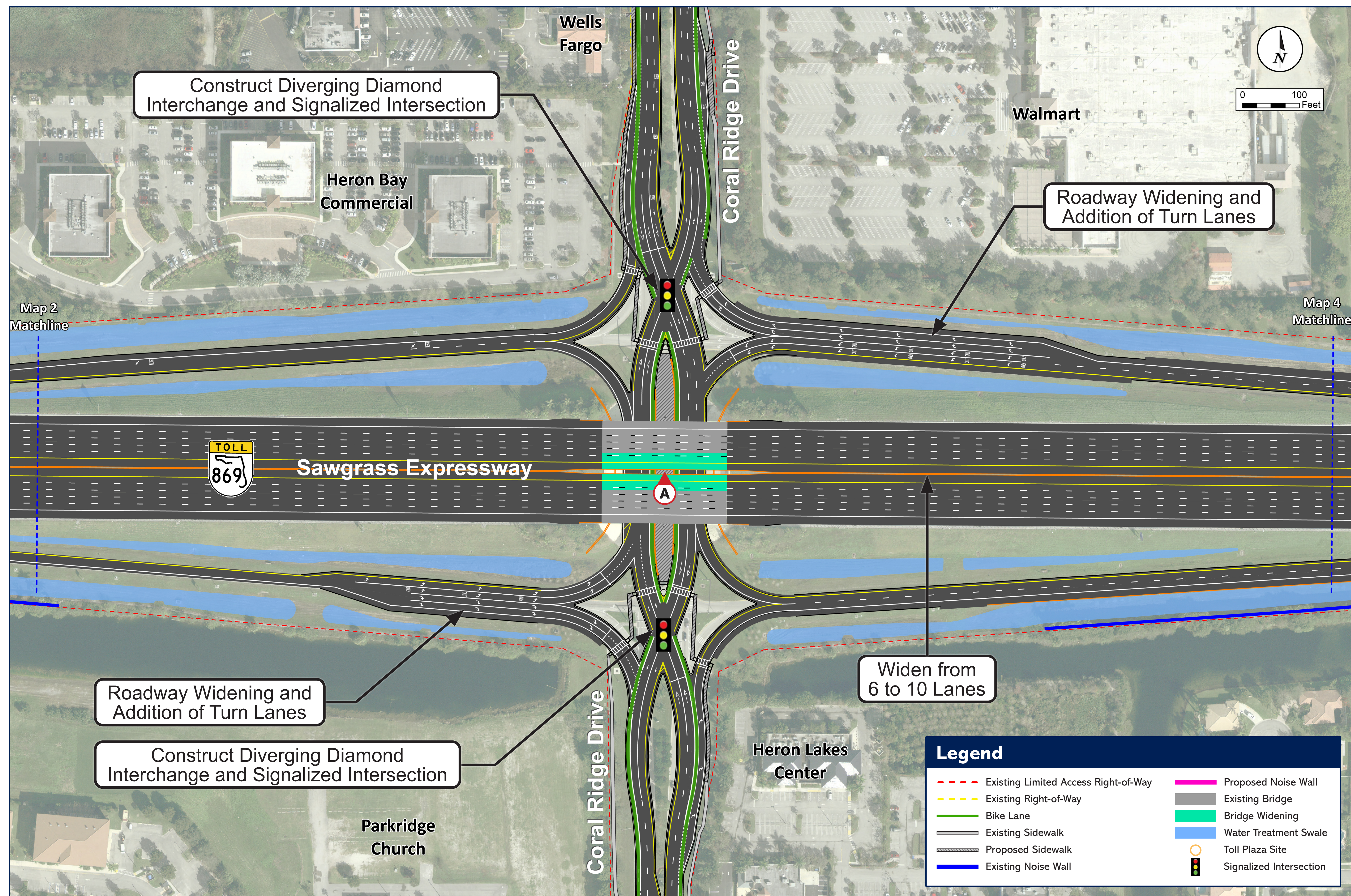
Coral Ridge Drive Interchange – North Section
