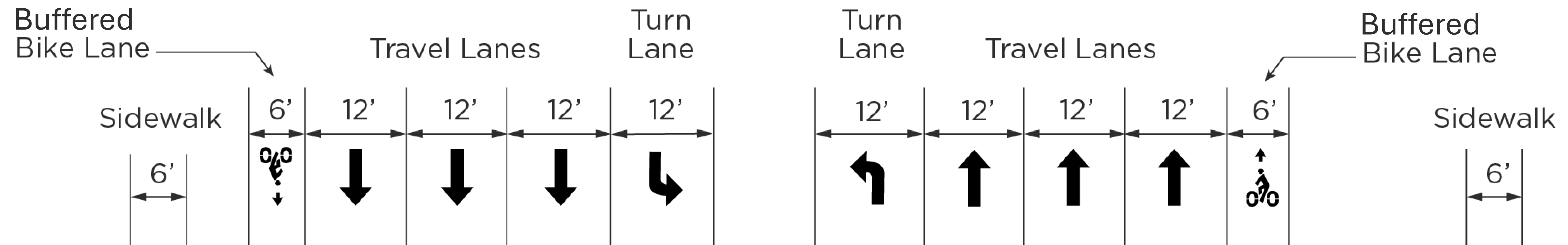
EXISTING TYPICAL SECTION
