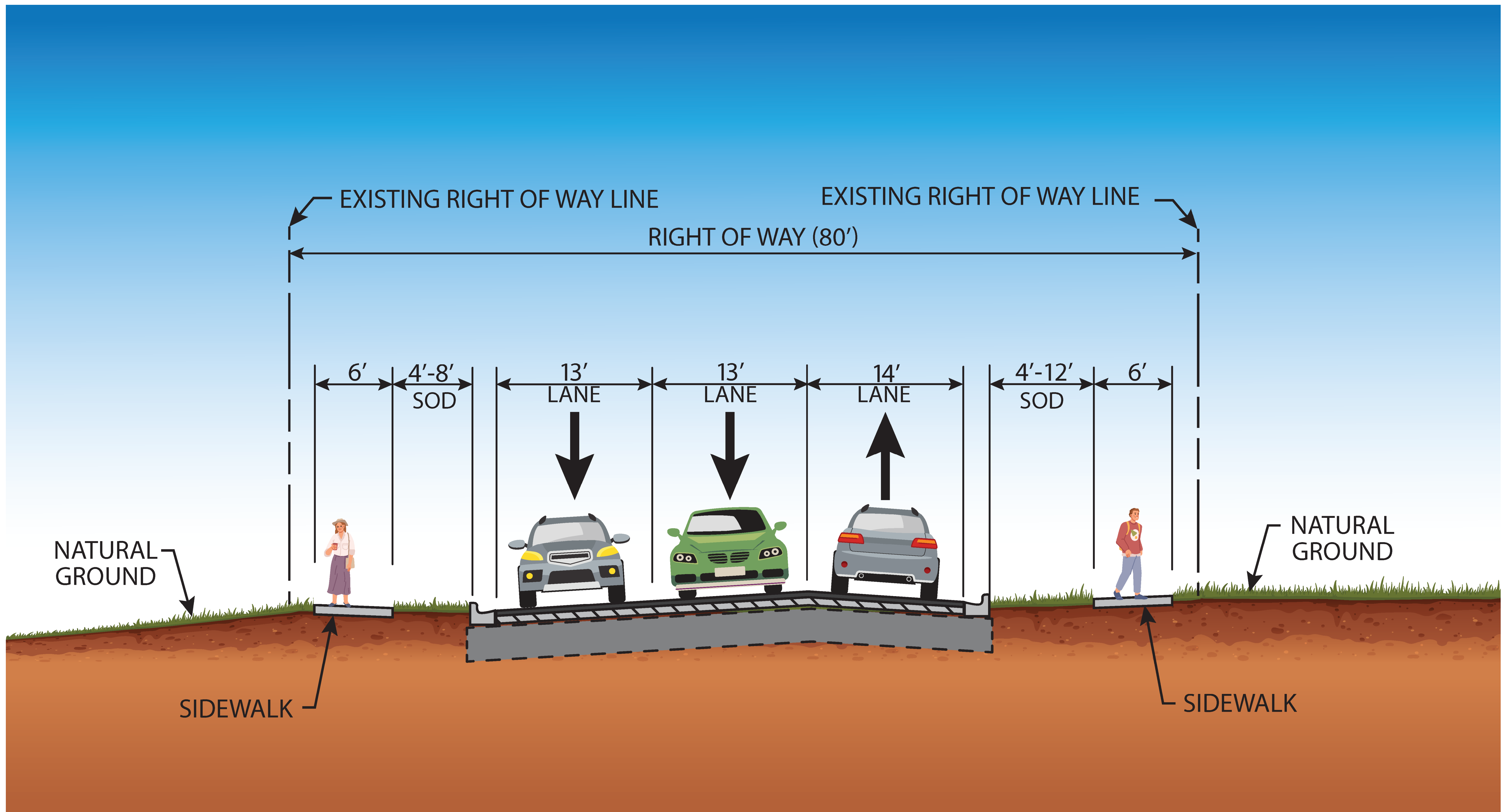
La Quinta Drive Typical Section (Looking East)
