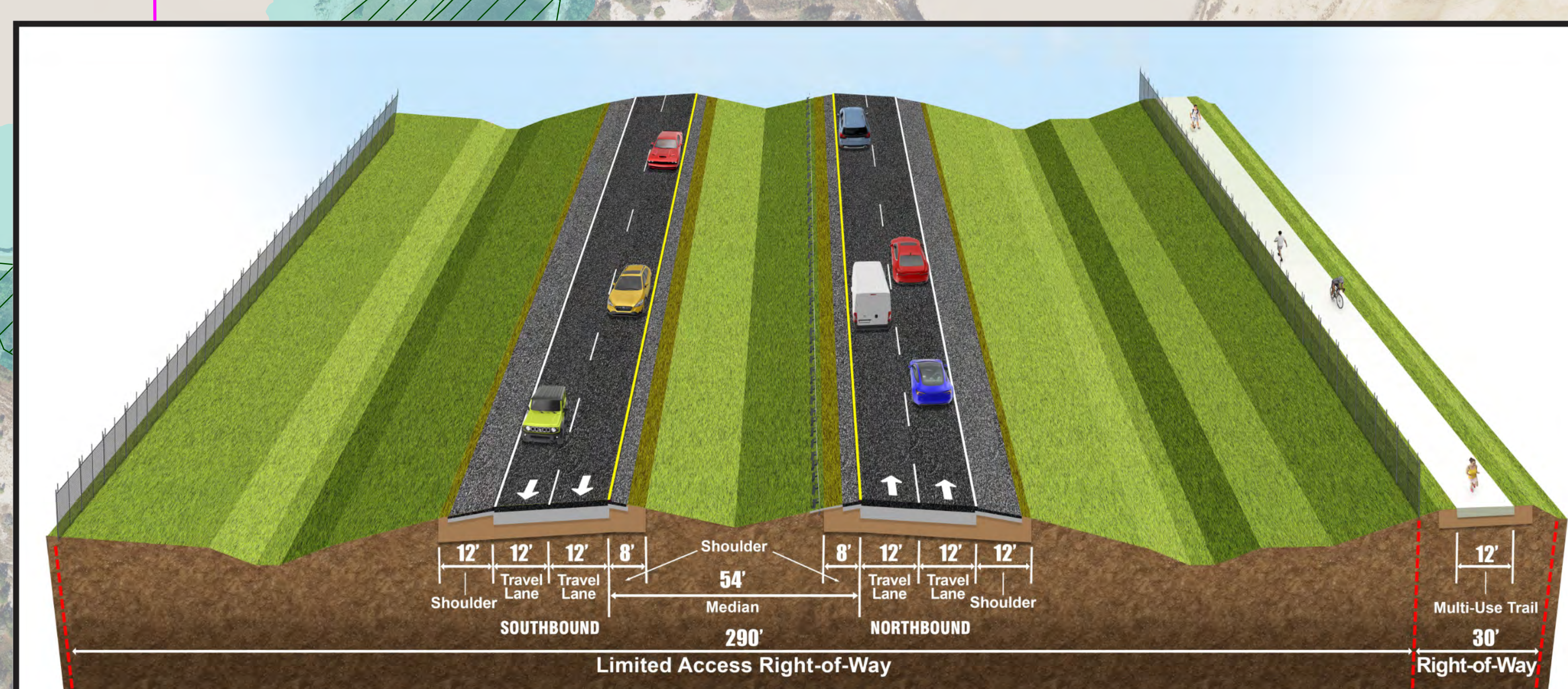
Proposed Typical Section of Central Polk Parkway Four-Lane Roadway
